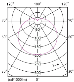
Light Distribution Diagram - Ess LEDBulb 10-75W E27 3000KA19 1PK
