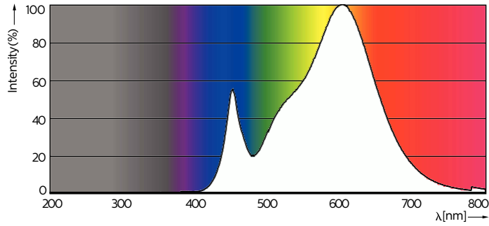
Spectral Power Distribution Colour - Ess LEDBulb 10-75W E27 3000K A19 1PK
