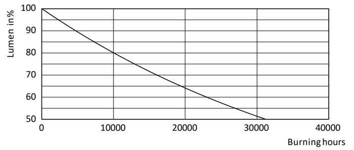
Lumen Maintenance Diagram - Ess LEDBulb 10-75W E27 6500K A19 1PK
