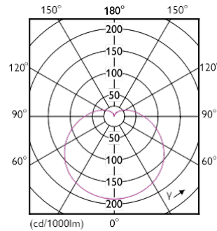
Light Distribution Diagram - Ess LEDBulb 12-100W E27 3000K A19 4PK
