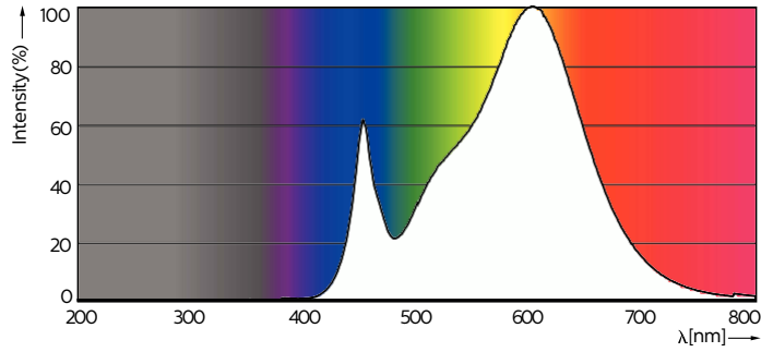
Spectral Power Distribution Colour - Ess LEDBulb 12-100W E27 3000KA19 4PK
