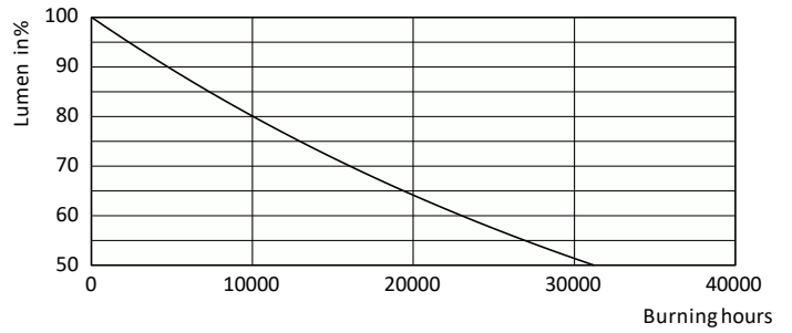
Lumen Maintenance Diagram - Ess LEDBulb 12-100W E27 3000KA19 4PK
