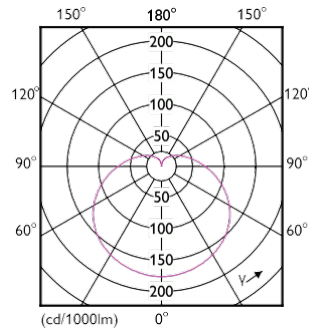
Light Distribution Diagram - Ess LEDBulb 8-60W E27 3000KA19 1PK
