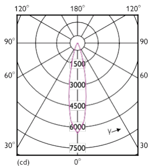
Light Distribution Diagram - PAR38 13-120W 930 25D 120V G ULW Dim E27
