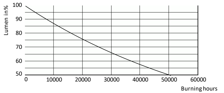
Lumen Maintenance Diagram - PAR38 13-120W 930 25D 120V G ULW Dim E27
