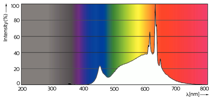
Spectral Power Distribution Colour - PAR38 13-120W 930 25D 120V G ULW Dim E27
