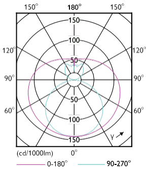
Light Distribution Diagram - CorePro LEDtube HO 1200mm 18W865 VVW T8
