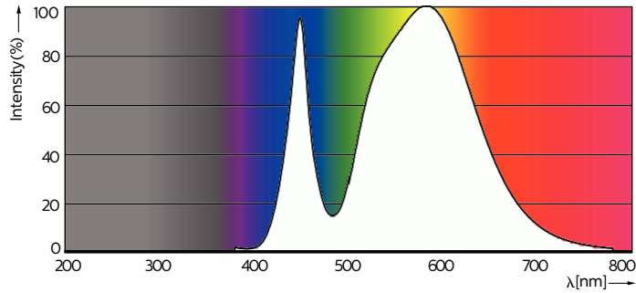
Spectral Power Distribution Colour - ECOFIT E LEDtube 1200mm 16W 740 T8 WV
