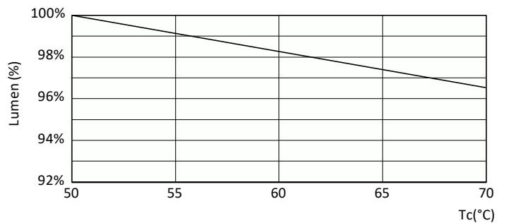
Lumen Maintenance Diagram - ECOFIT E LEDtube 1200mm 16W 765 T8 WV
