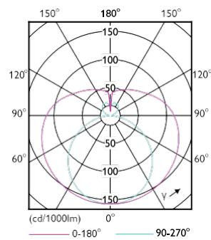
Light Distribution Diagram - ECOFIT E LEDtube 600mm 8W 765 T8 WV
