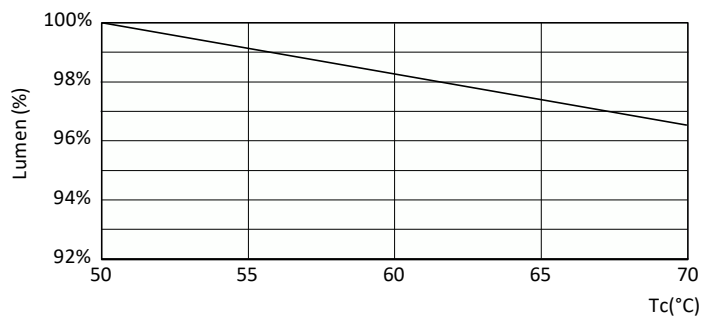
Lumen Maintenance Diagram - ECOFIT E LEDtube 600mm 8W 765 T8 WV
