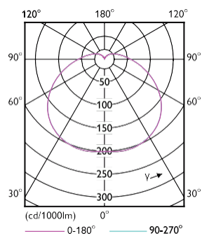
Light Distribution Diagram - TForce Core HB 3Klm 40W E27 865 WV
