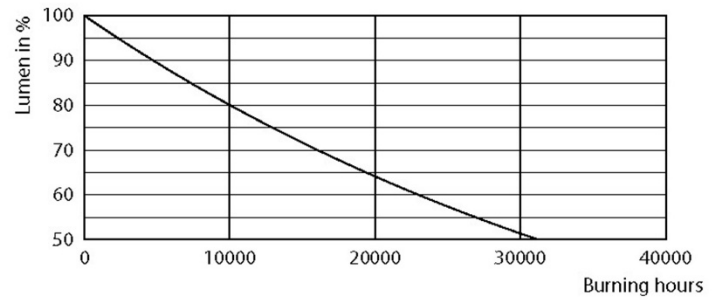
Lumen Maintenance Diagram - TForce Core HB 4Klm 50W E27 865 WV
