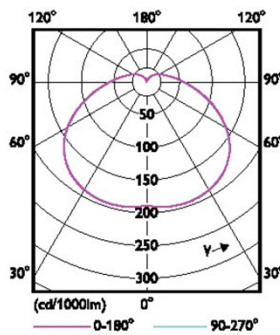
Light Distribution Diagram - TForce Core HB 4Klm 50W E27 865 WV
