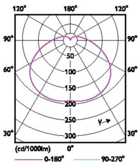
Light Distribution Diagram - TForce Core HB 4Klm 50W E40 865 WV
