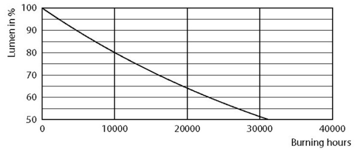
Lumen Maintenance Diagram - TForce Core HB 4Klm 50W E40 865 WV
