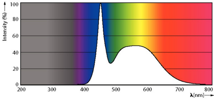
Spectral Power Distribution Colour - TForce Core HB 4Klm 50W E40 865 WV
